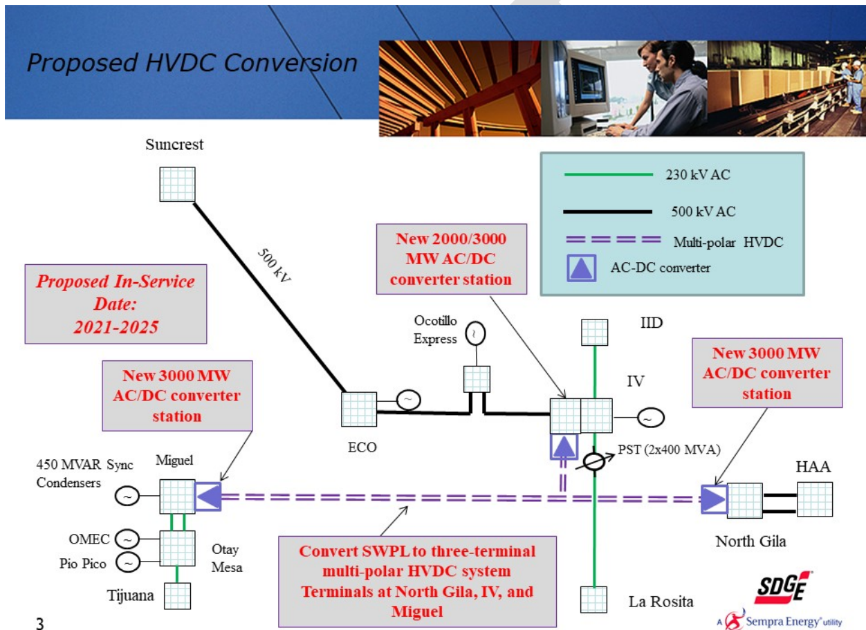
Figure 1: Project Map (Source: HVDC Conversion Project Summary)
